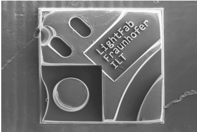
Image 3: Fine structure (approximately 400 x 400 μm) produced with the new process combination and attached to a solid base (see Image 2). © Fraunhofer ILT, Aachen, Germany.
